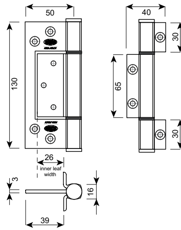
Overall dimensions
