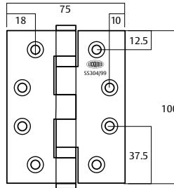
Overall dimensions
